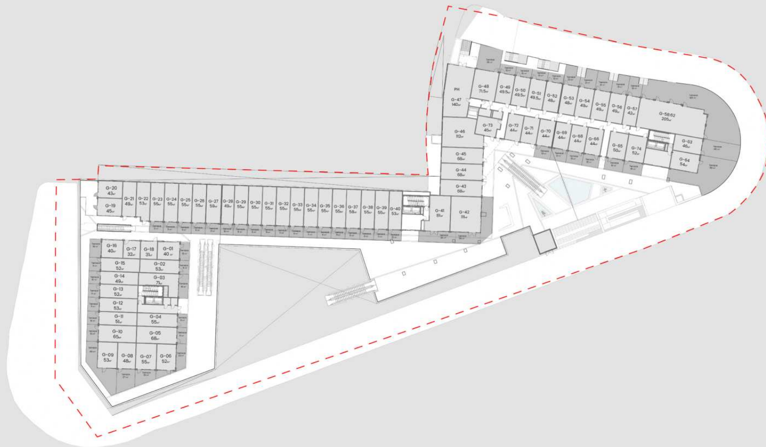
Ground Floor
